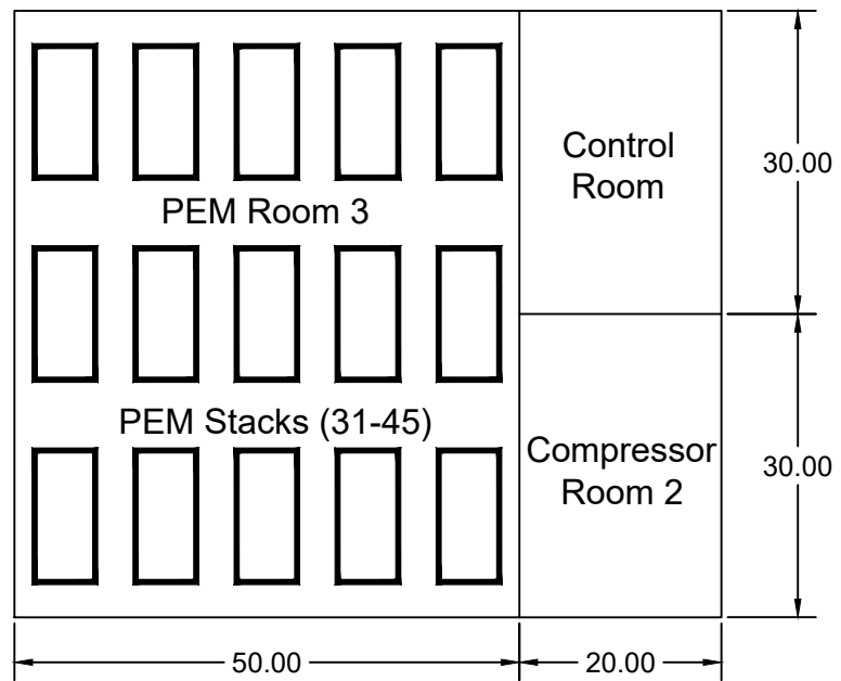
3RD DECK @ ELV 32 m AWL
