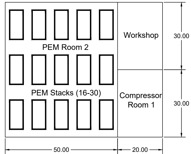
2ND DECK @ ELV 28.5 m AWL
