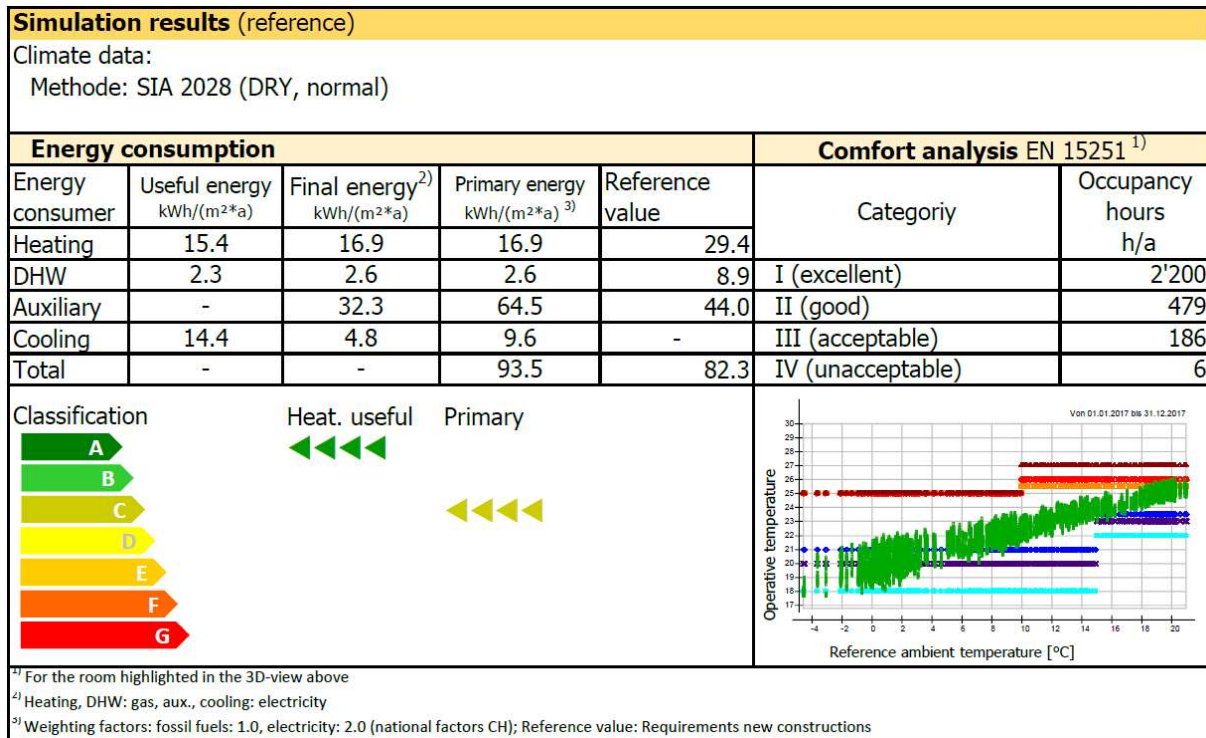
Figure 6: Simulation results for a typical Swiss office building with standard TMY meteo data.
