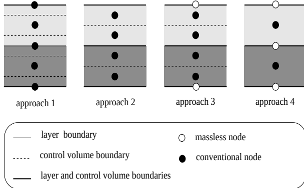
Figure 6: Control Volume Nodal Schemes
