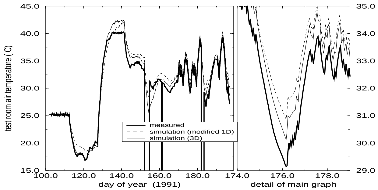
Figure 8: Measured, Modified 1-D and 3-D Air Temperatures
