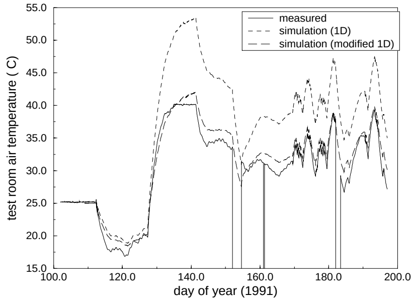
Figure 5: Measured, 1-D and Modified 1-D Air Temperatures
