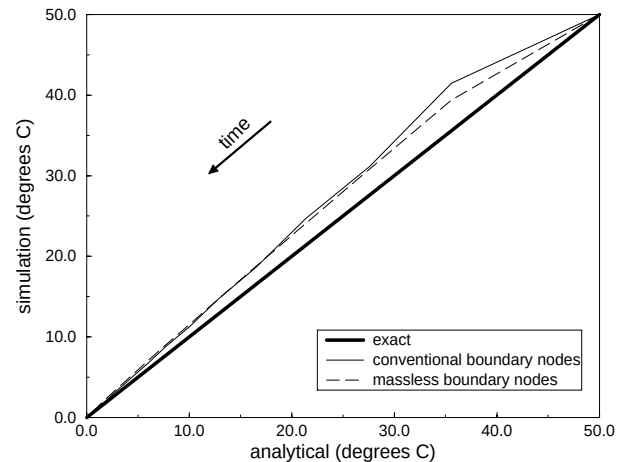
Figure 7: Analytical Comparison: Decay from Step Change
