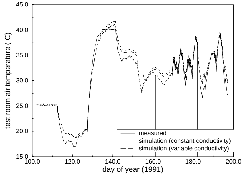
Figure 9: Effect of Conductivity Temperature Dependence
