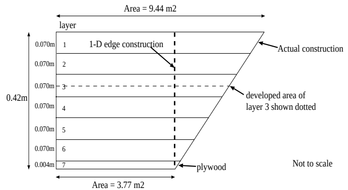
Figure 4: Geometry of the Developed Area
