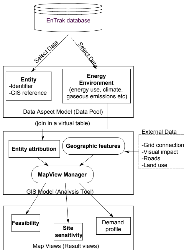
Figure 5 The data connectivity and procedure of GIS-based energy data views.
