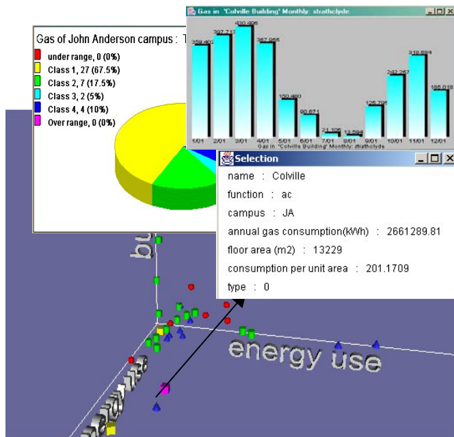
Figure 4 Integrated analysis support by EnTrak in coherent manner.
