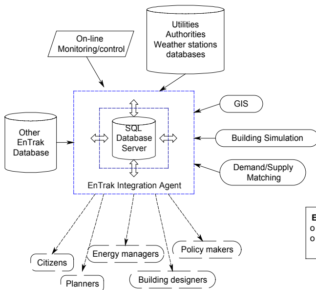
Figure 1 Architecture of EnTrak.
