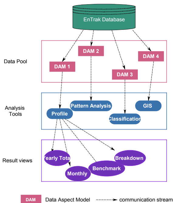
Figure 3 Portable data aspect models supporting multi-scales analysis model.
