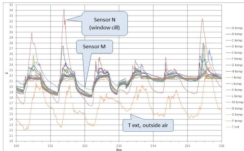
Figure 5: Temperature profiles during a warm period from all sensing points.
