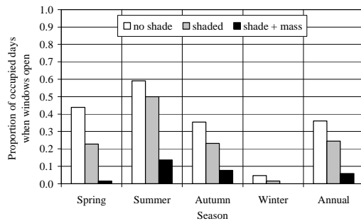
Figure 11 Predicted window opening v. building design option.
