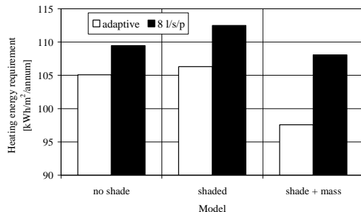
Figure 12 Annual heating energy demand for each design option modeled using the Humphreys algorithm (adaptive) and the fixed ventilation rate method (8l/s/p).
