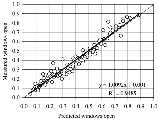
Figure 2 Predicted v. Observed window openings.
